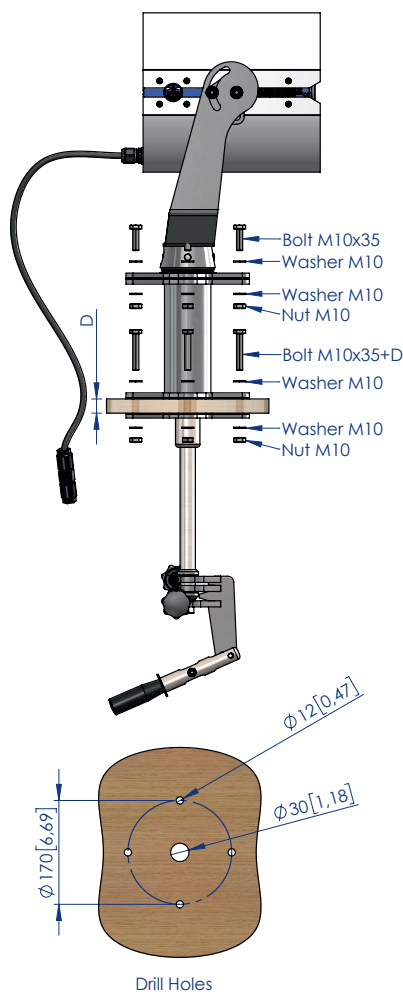
1 Mounting the searchlight
