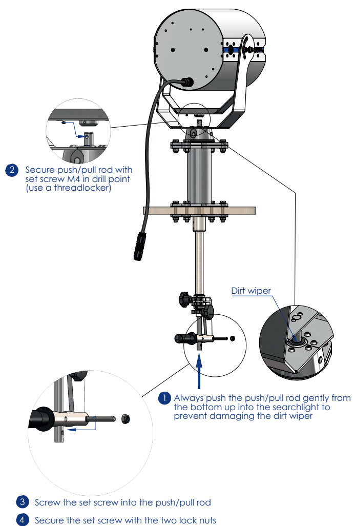
2 Installing the push/pull rod
